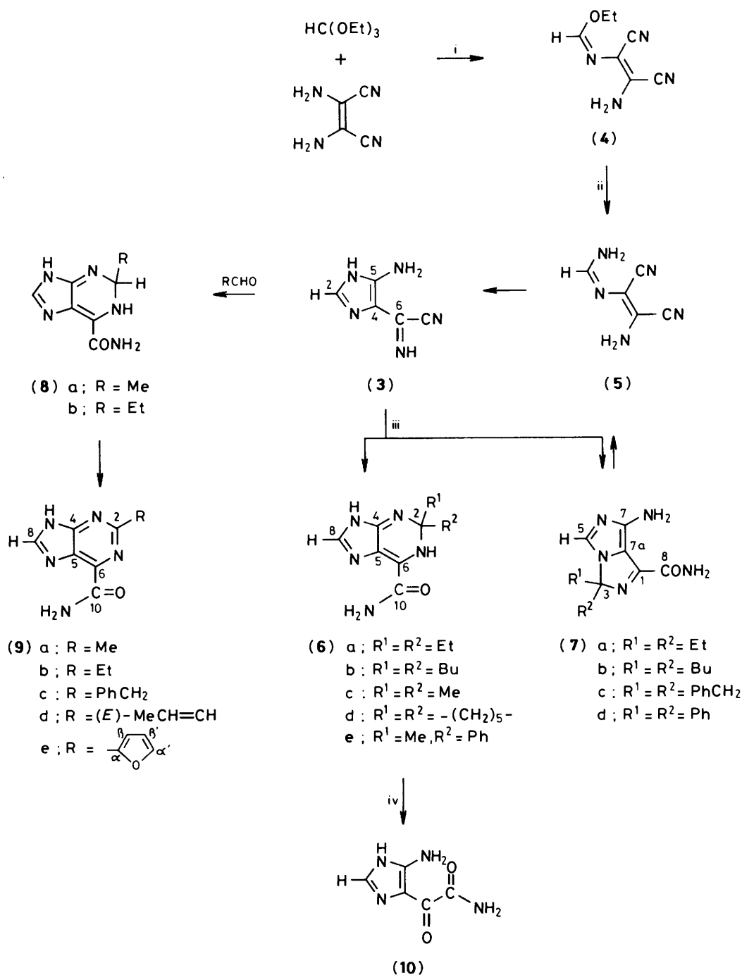
Scheme 2. Reagents and conditions: i, dioxane; ii, NH 3 , -78 °C, PhNH 3 + Cl - ; iii, R 1 R 2 CO; iv, SiO 2 or MeOH aq.
